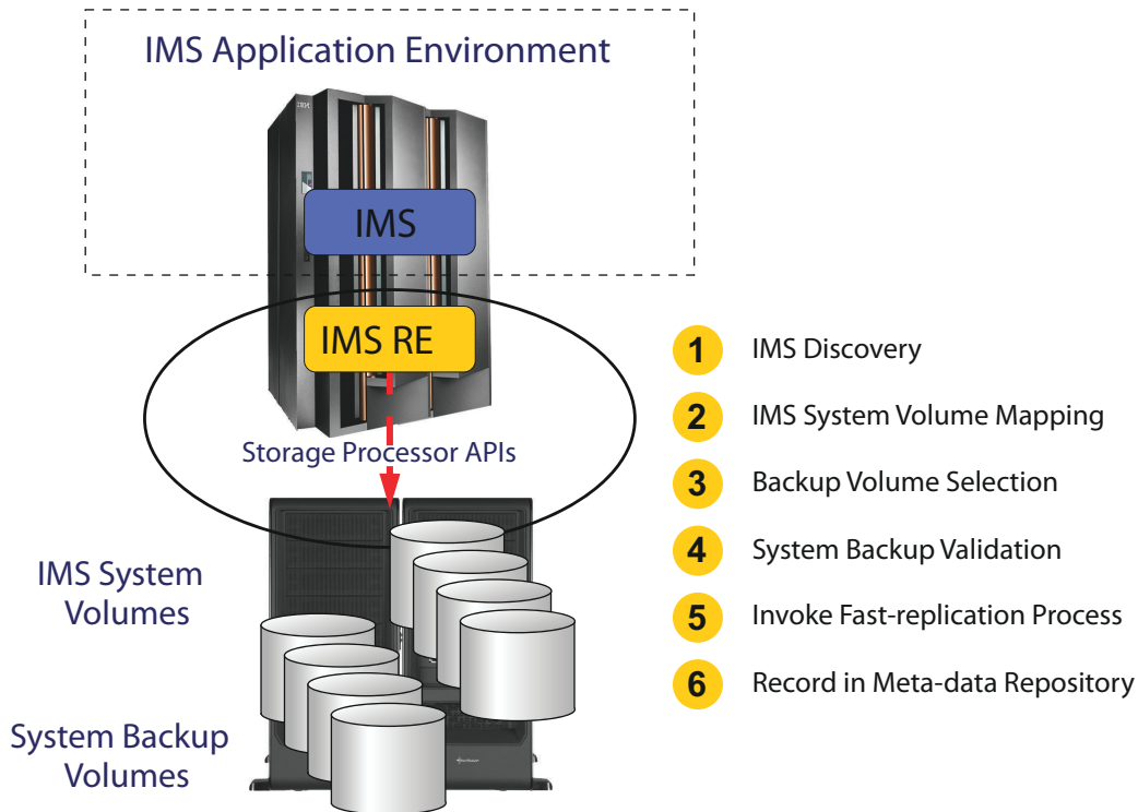
Figure 4. Creating an IMS full System Level Backup
