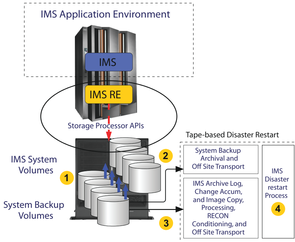
Figure 7. Using IMS Recovery Expert to implement a tape-based disaster restart methodology
