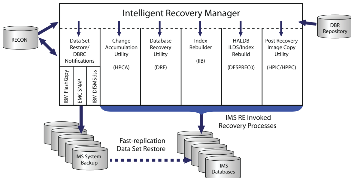
Figure 6. IMS Recovery Expert controlled application recovery
